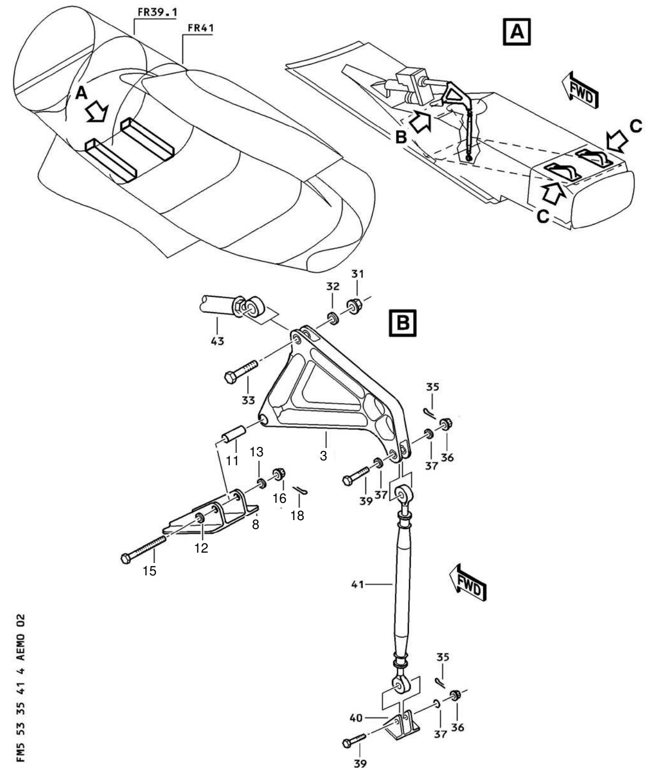
Air Inlet Flap - Component Location Figure 402/TASK 53-35-41-991-002- 12 (SHEET 1)
