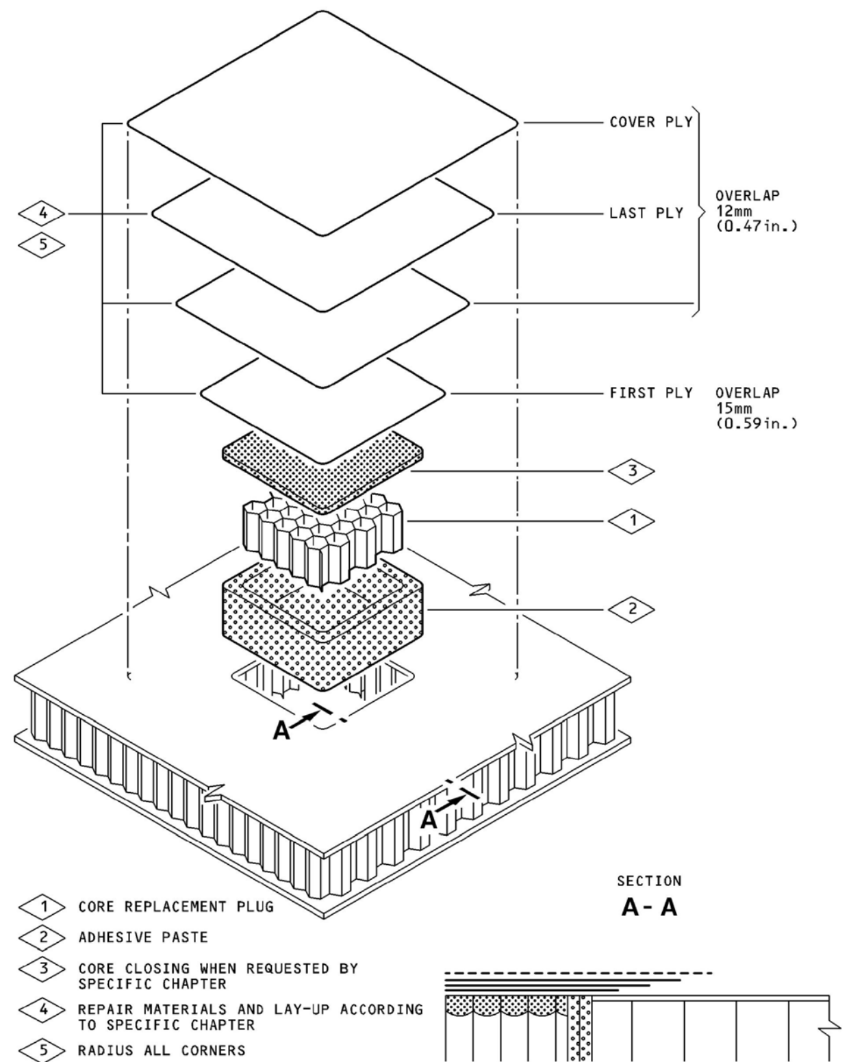
Wet Lay-Up Repair - one skin damaged Option D Figure 2 (sheet 4)
