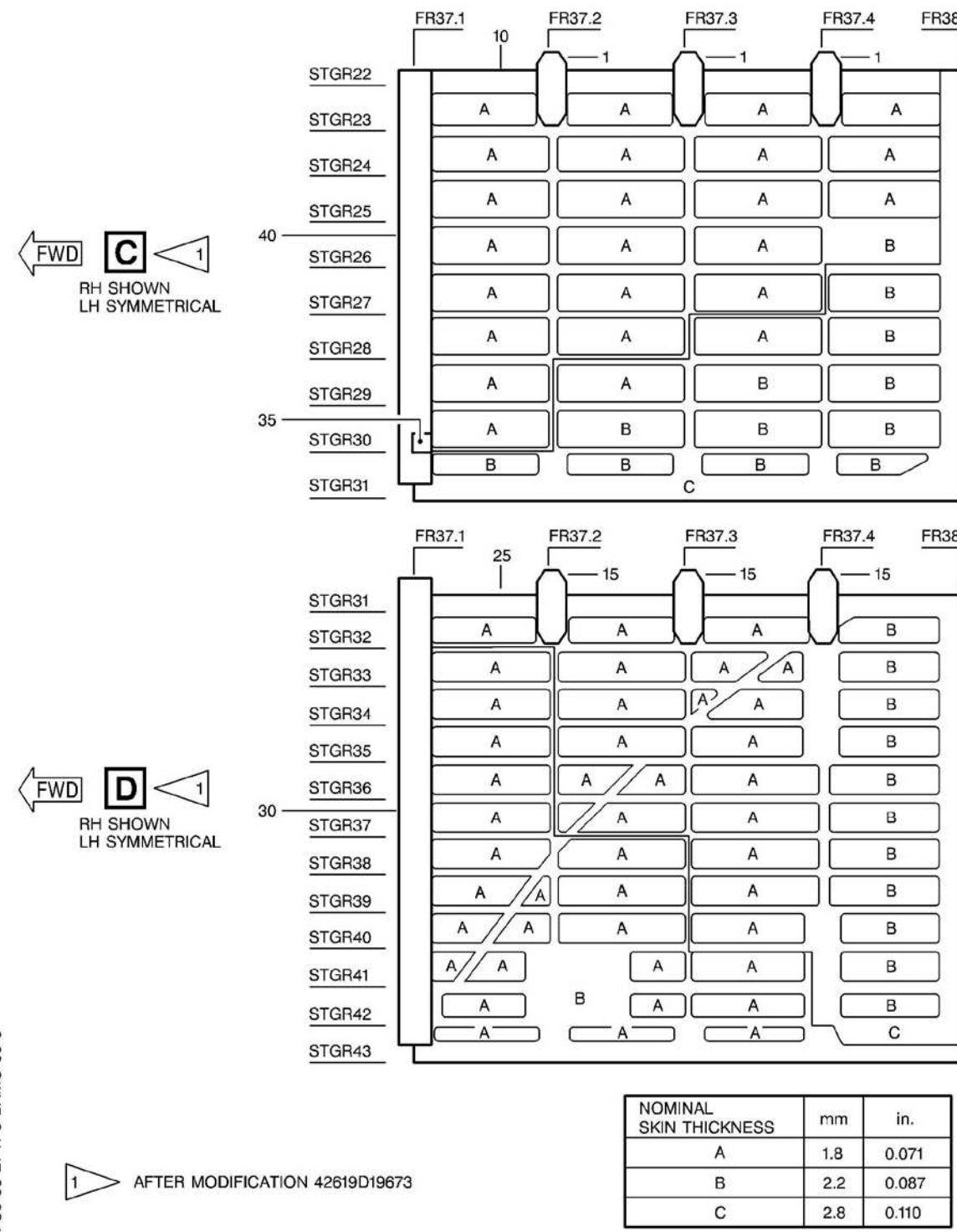
FR37.1-FR38, STGR22 thru STGR43, Skin Panels, Straps and Buttstraps Figure 14 (sheet 2)
