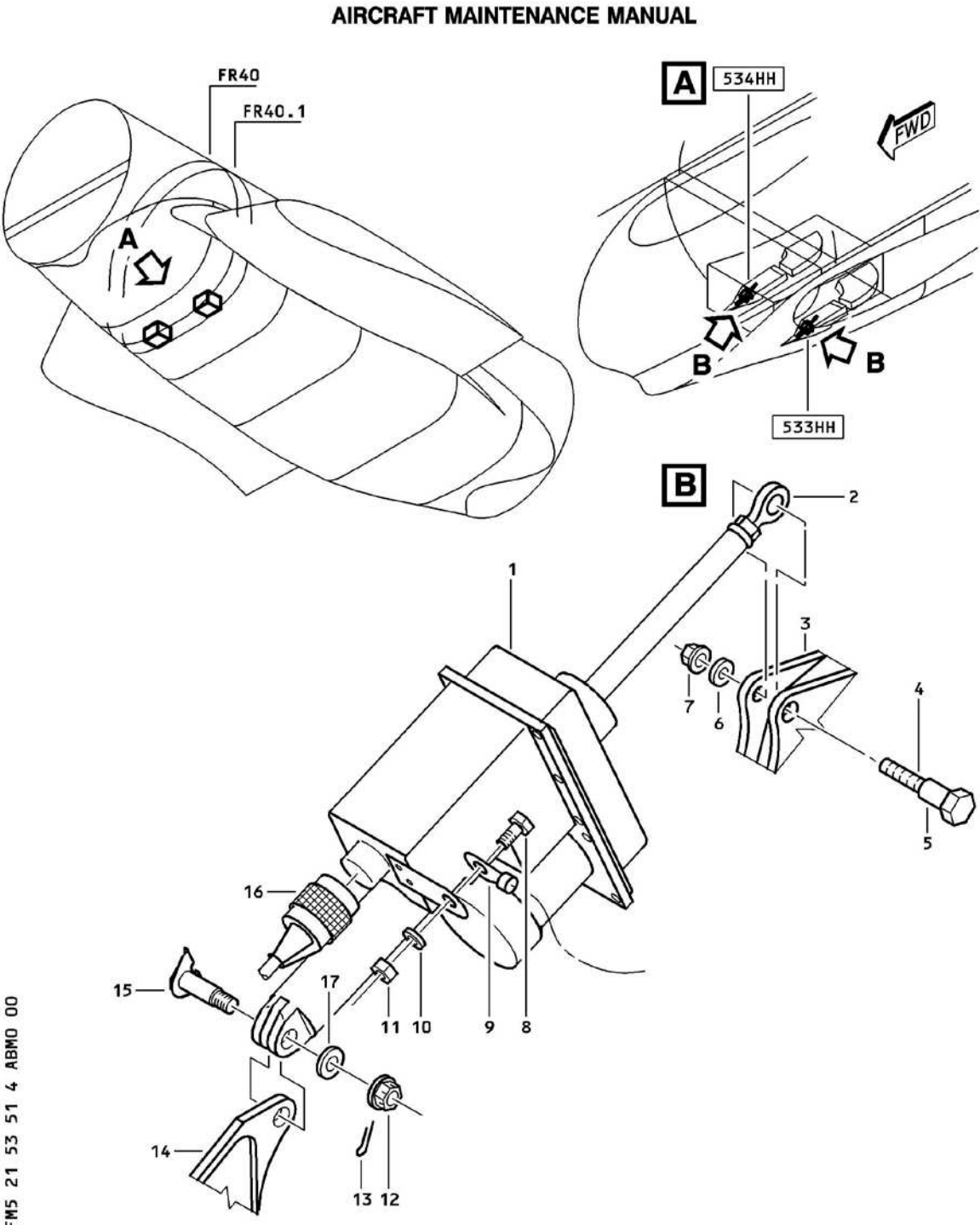
Air-Inlet Flap Actuator Figure 401/TASK 21-53-51-991-001-A
