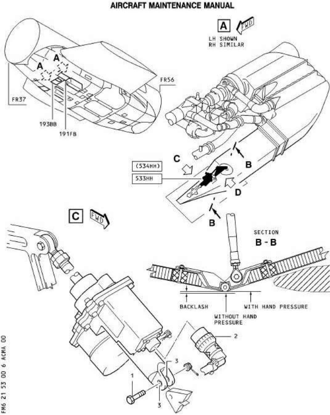
Inspection Control Points Figure 602/TASK 21-53-00-991-006- 12 (SHEET 1)
