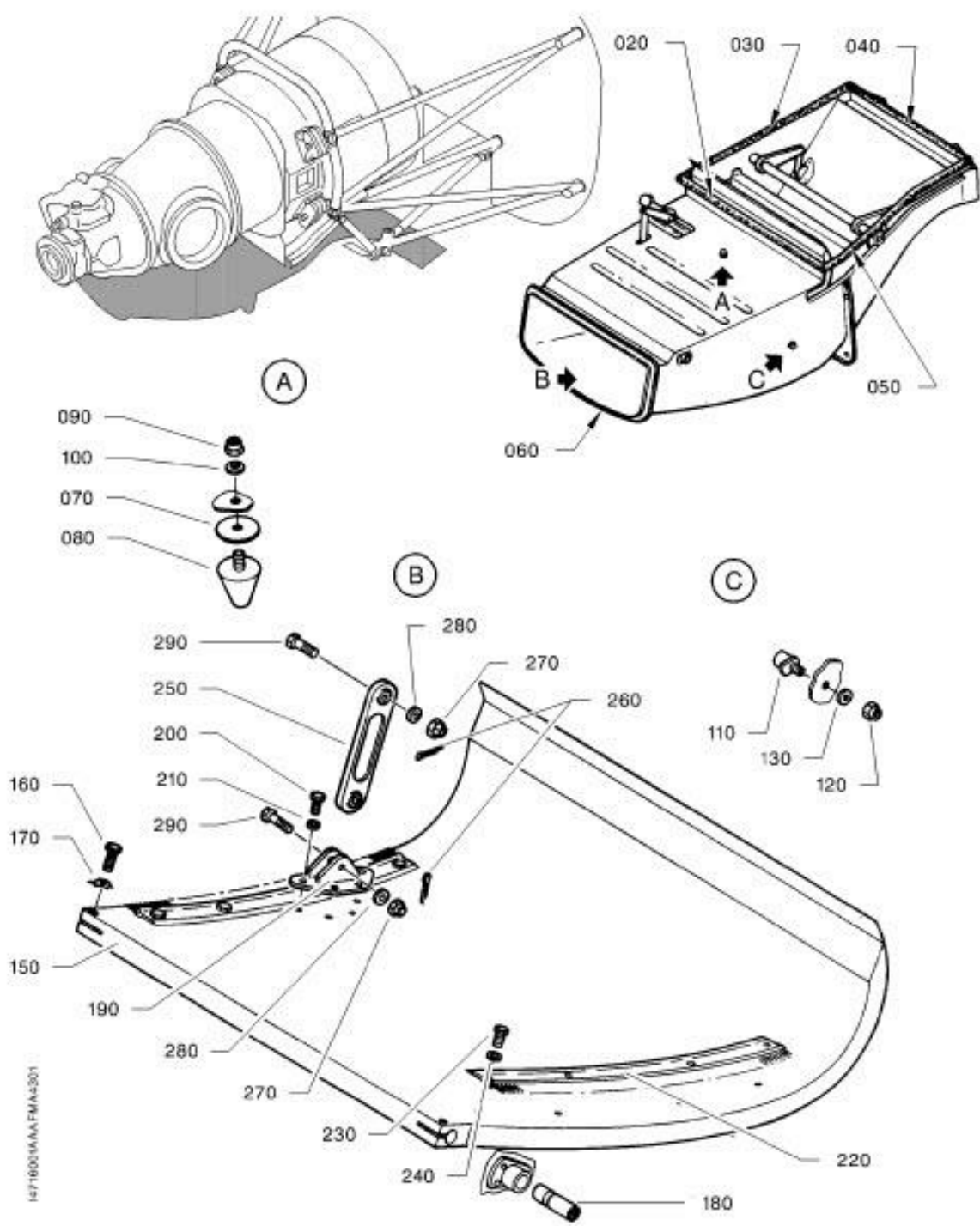
INERTIAL SEPARATOR - FLAP FIGURE 2
